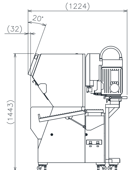
RIGHT VIEW
