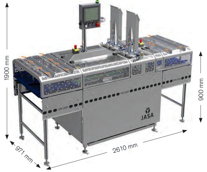
JSPGS2100 Dual Lane Sleever with Safety Infeed / Outfeed
