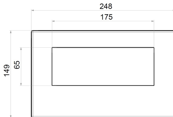
Front View Dimensions (mm)
