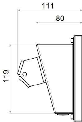
Side View Dimensions (mm)
