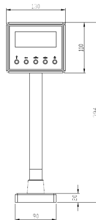
SCALE INDICATOR FRONT VIEW
